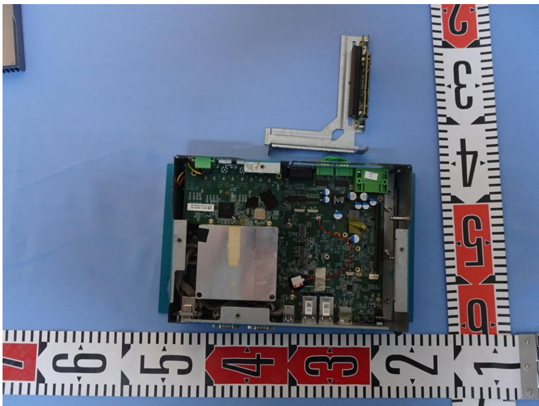
Photograph 6 – Internal view
