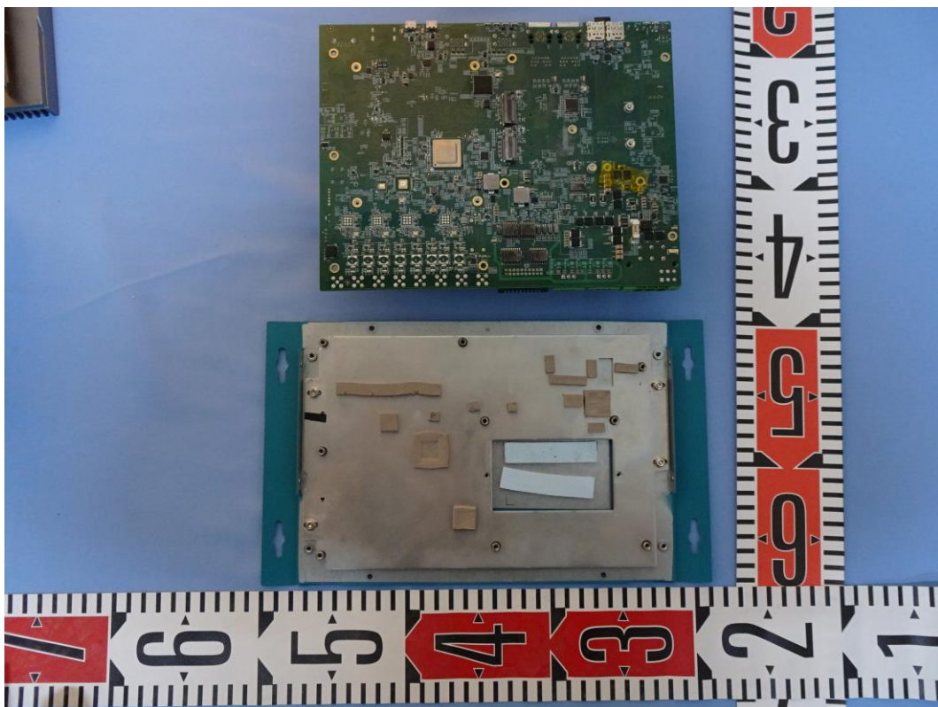
Photograph 8 – Internal view
