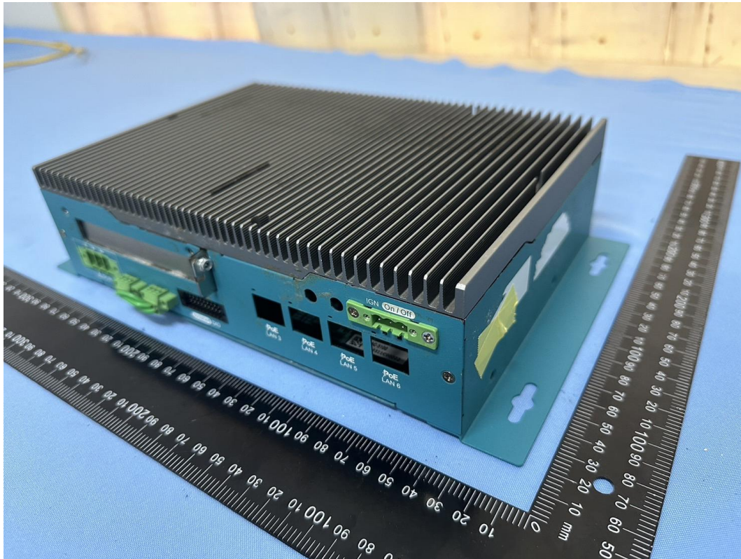
Photograph 1 – External view
